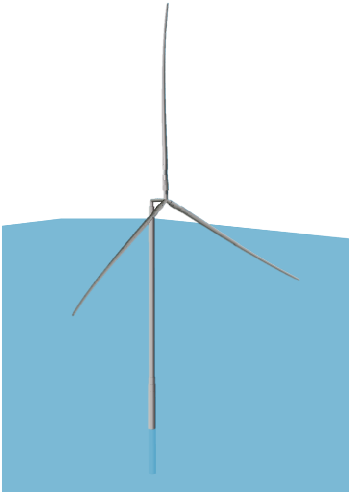
25MW Offshore Wind Turbine Reference Model
